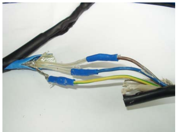
Heating cable Type VCD 17/1425
